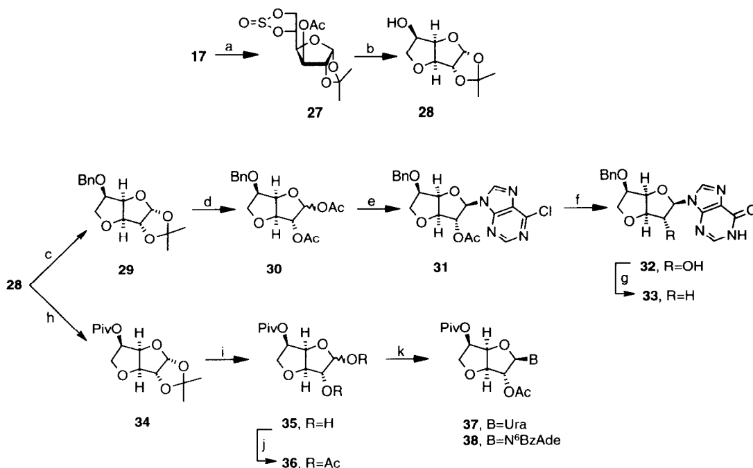
Scheme 3. a) Ref. 16a; b) NaOMe, MeOH, 0°C → r.t., 30 min (97%); c) NaH, BnBr, THF, r.t., 5 h (84%); d) AcOH, H 2 SO 4 , Ac 2 O, r.t., 5 h (74%); e) BSA, TMSOTf, Cl 2 C 2 H 4 , 6-chloropurine, reflux, 40 min (64%); f) HSCH 2 CH 2 OH, MeOH, NaOMe, reflux, 4 h (87%); g) CH 3 CN, DMAP, PhOCSOCl, r.t., 3 h, then toluene, AIBN, n -Bu 3 SnH, reflux, 3.5 h (42%); h) PivCl, pyridine, DMAP, r.t., 24 h (98%); i) 80% aq. AcOH, 120–125°C, 4 h (83%); j) Ac 2 O, pyridine, r.t., overnight (93%); k) BSA, TMSOTf, Cl 2 C 2 H 4 , uracil or N 6 -benzoyladenine, reflux, 40–45 min (80%).
