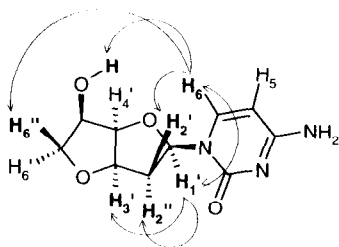
Figure 2. NOE experiments
