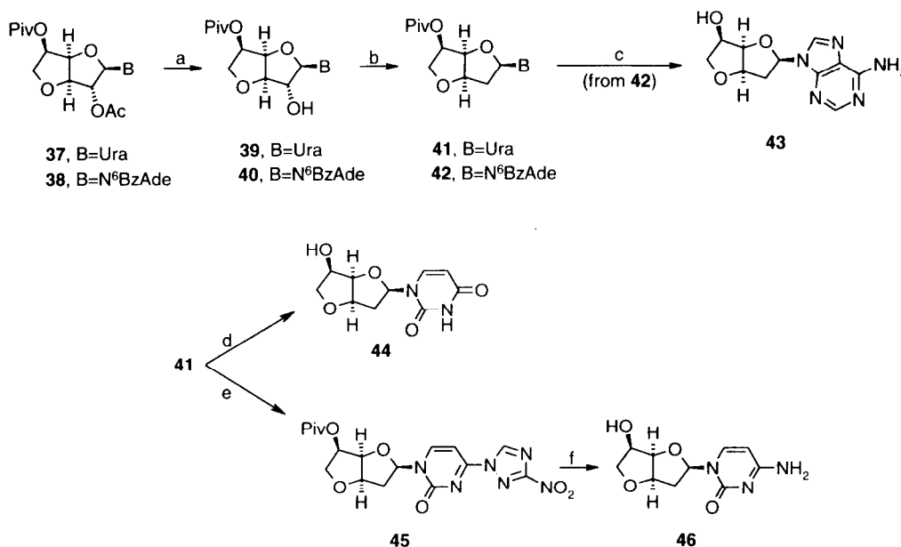
Scheme 4. a) MeOH/NH 3 (10–20%), r.t., 50 min–3 h (85–99%); b) i: CH 3 CN or Cl 2 C 2 H 2 , DMAP, PhOCSCl, r.t., 40 min–4 h. ii: Toluene, AIBN, n -Bu 3 SnH, reflux, 50 min–1.5 h (63–80%); c) Conc. aq. NH 3 soln., 55–60 °C, 8 h (67%); d) Basic resin Amberlite IRA-402, MeOH, r.t., 16 h (quantitative); e) Pyridine, MSNT, diphenylphosphate, r.t., 8 h (66%); f) MeOH/NH 4 OH conc., r.t., 3 days, (91%).
